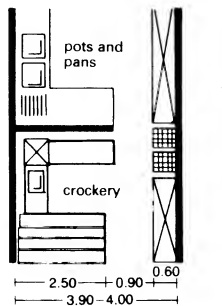
9 Crockery and pan washing
